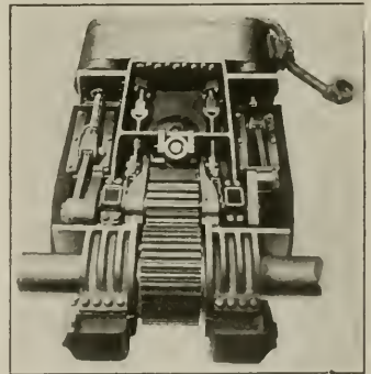
TWO-CYLINDER ENGINE GEARED TO THE TRAILER AXLE
